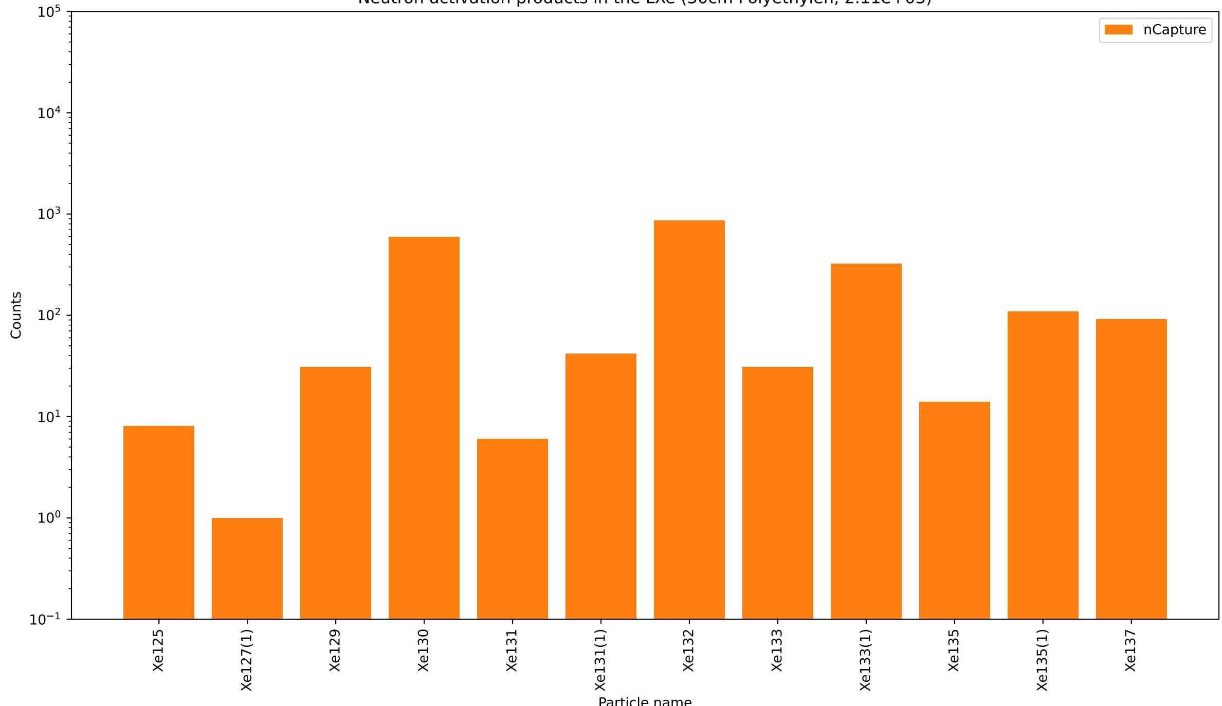
Neutron activation products in the LXe (30cm Polyethylen, 2.11e+03)
