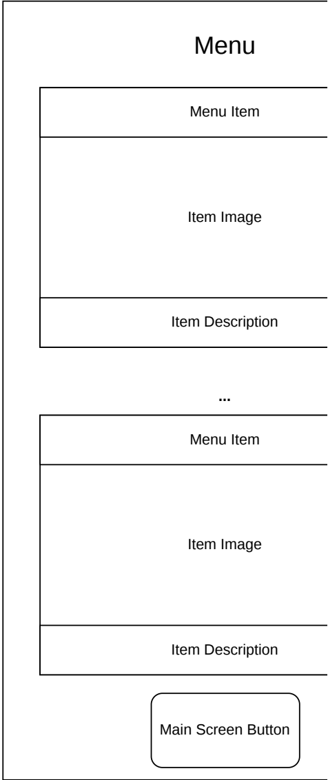
Menu Screen
