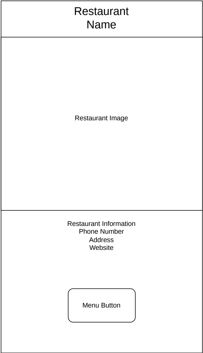
Main Screen
