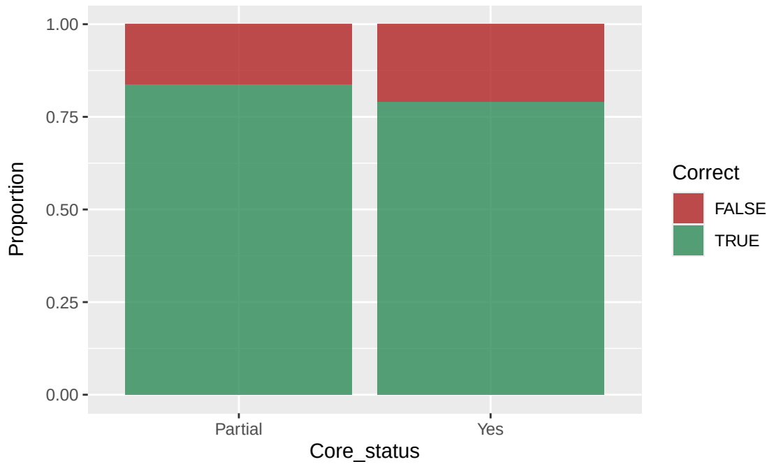
Core_status
