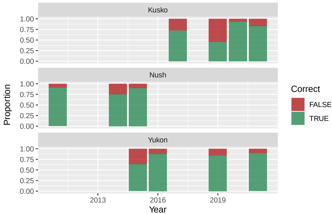
Core_status
