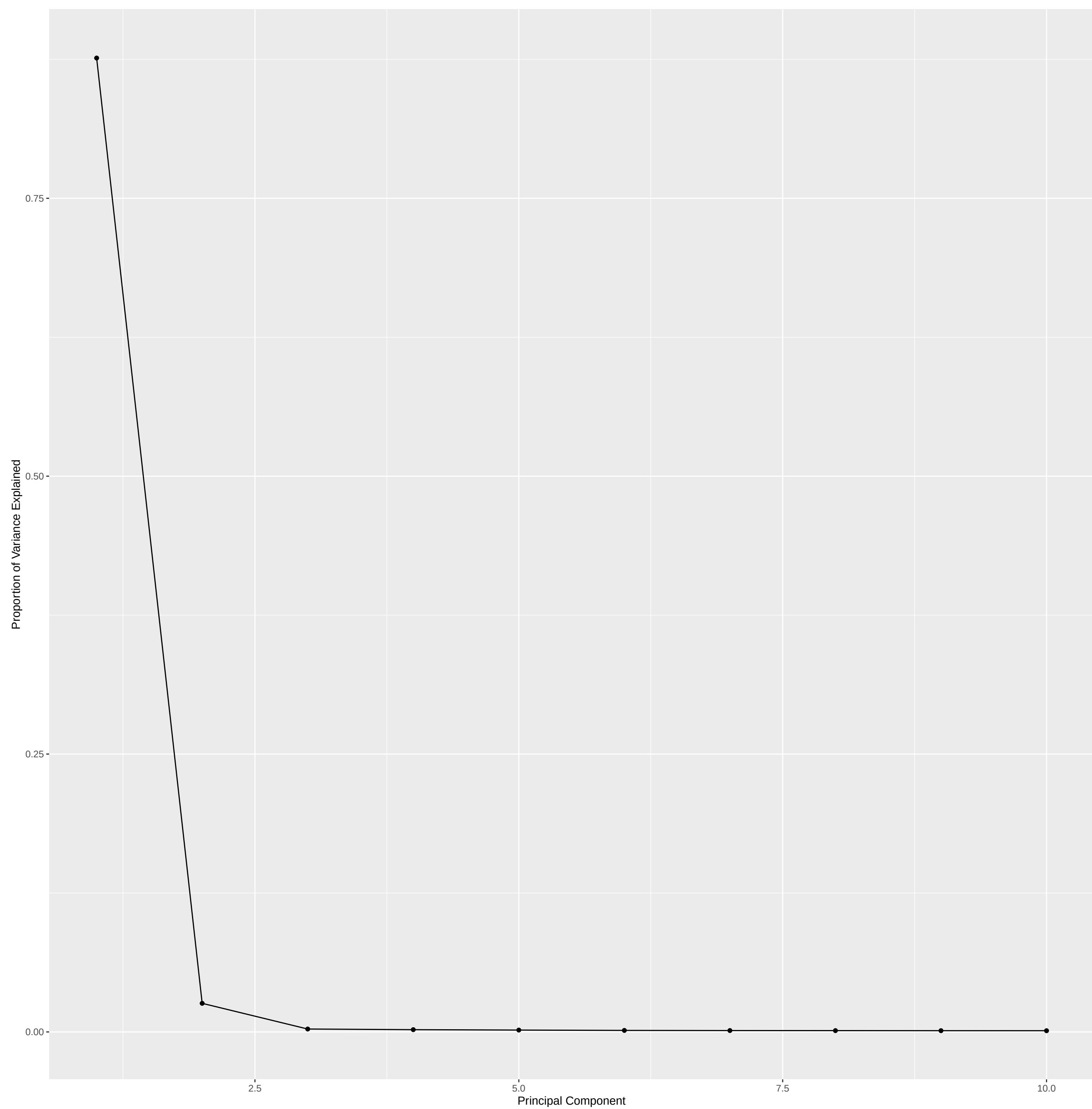
Scree Plot (First 10 Components)
