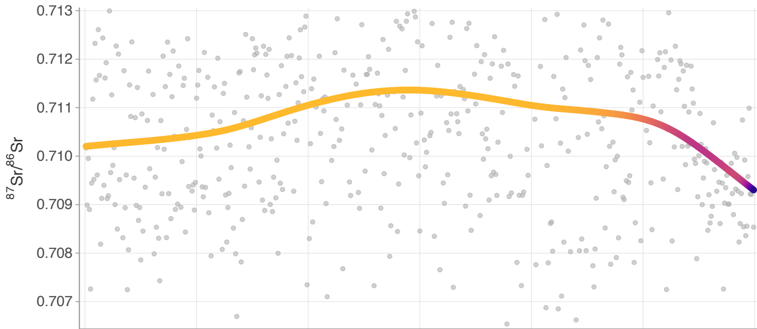
PC1 (92.2%)
