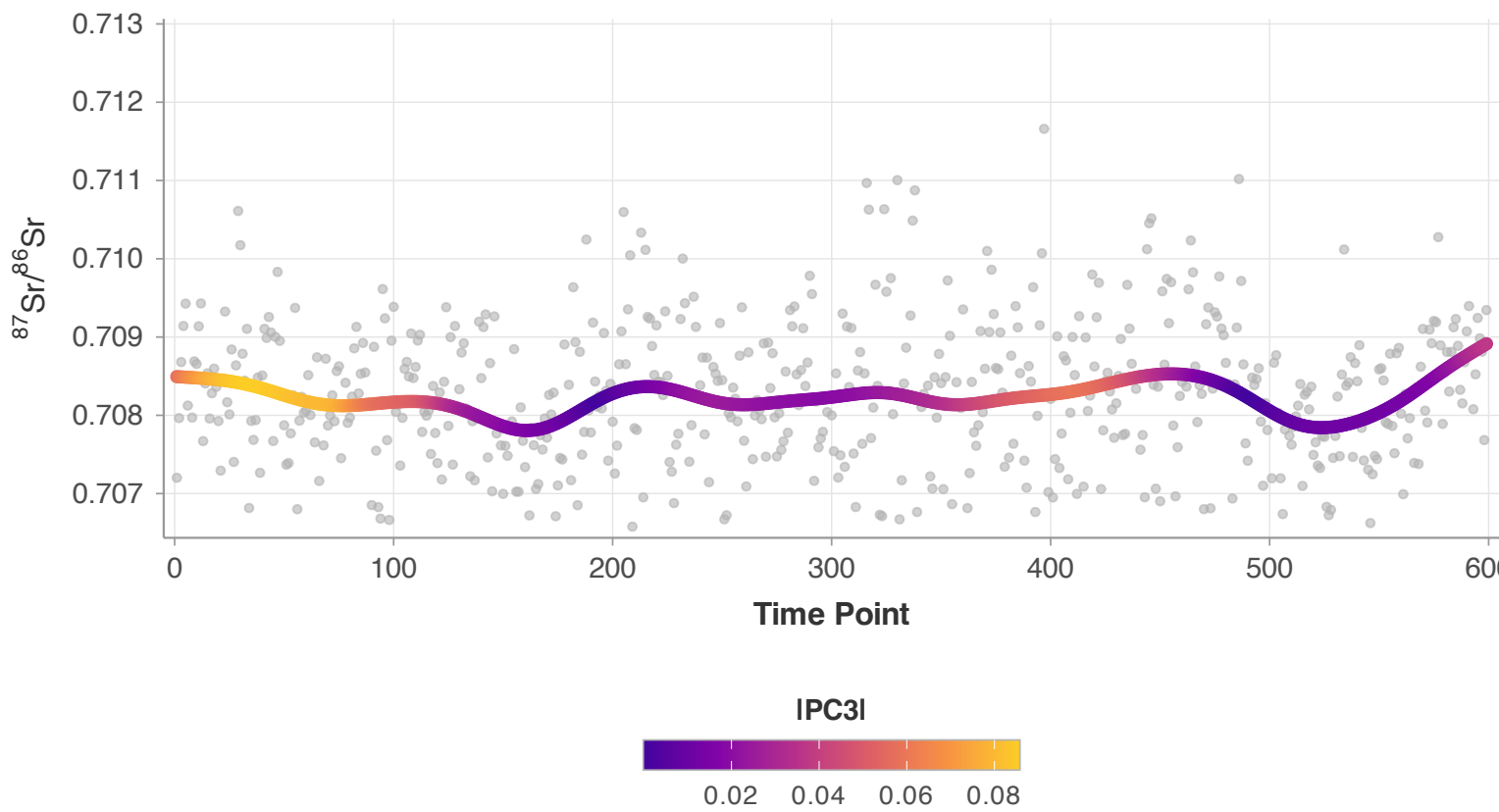
PC3 (10.2%)
