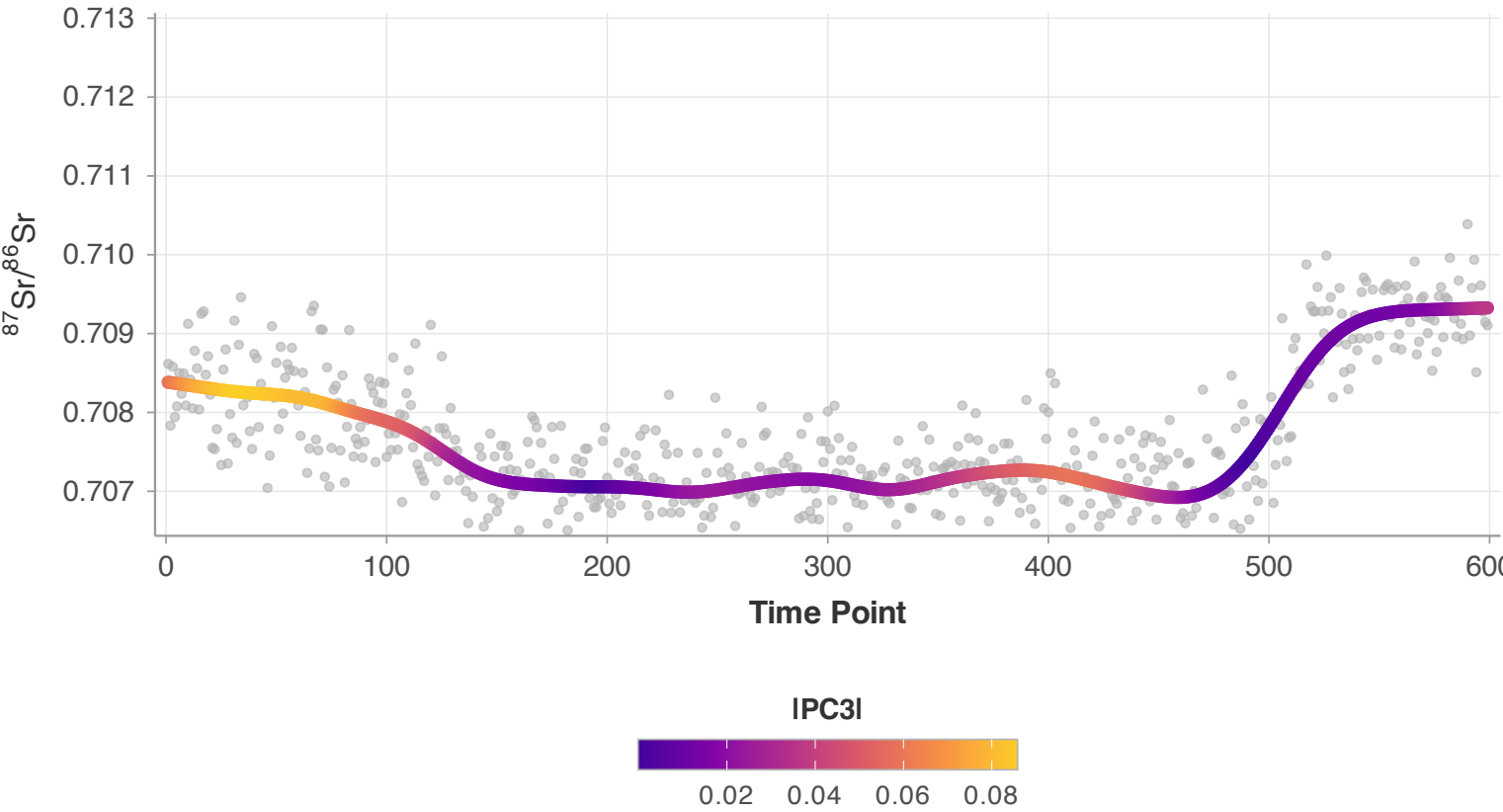
PC3 (10.2%)
