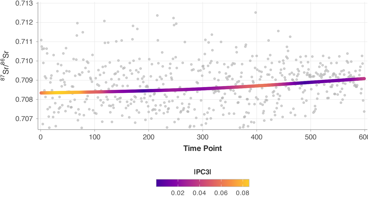
PC3 (10.2%)
