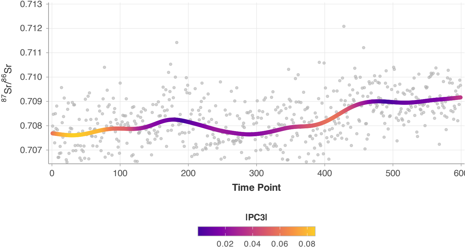
PC3 (10.2%)
