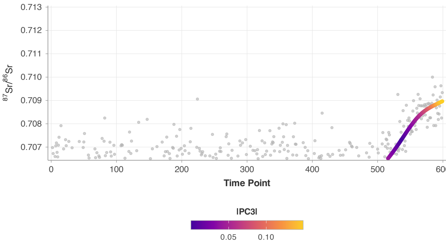
PC3 (1.1%)
