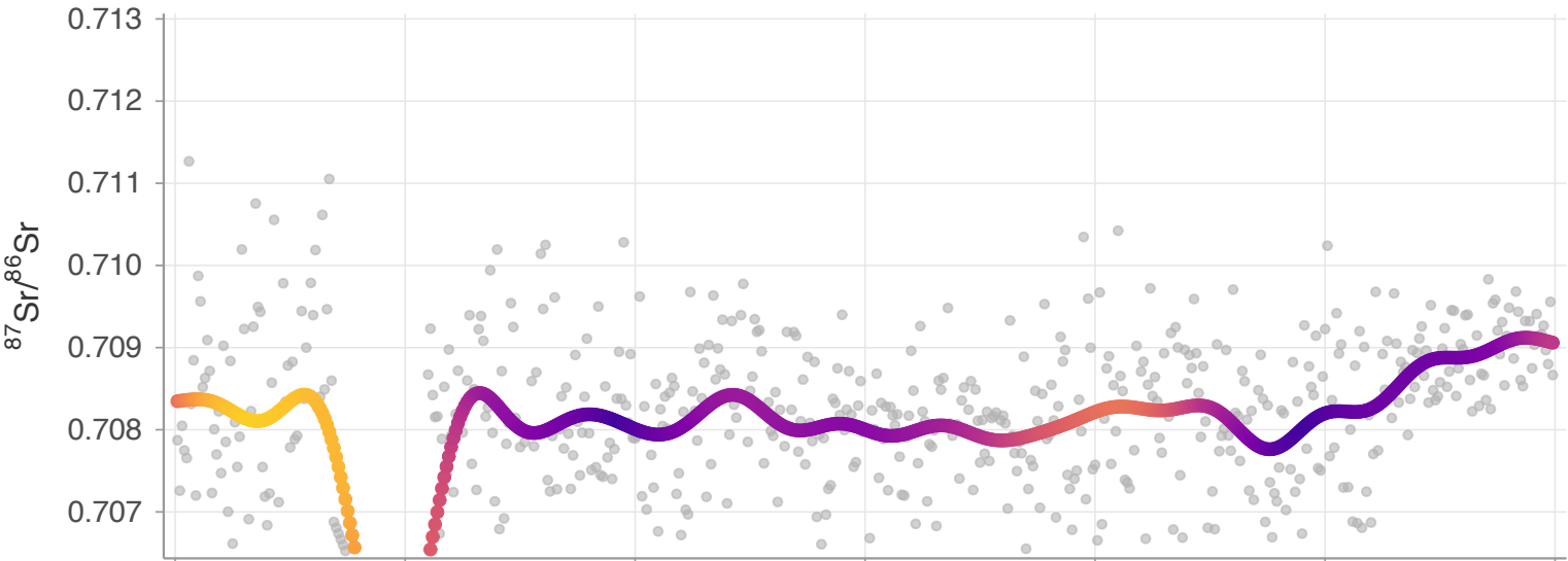
PC3 (10.2%)
