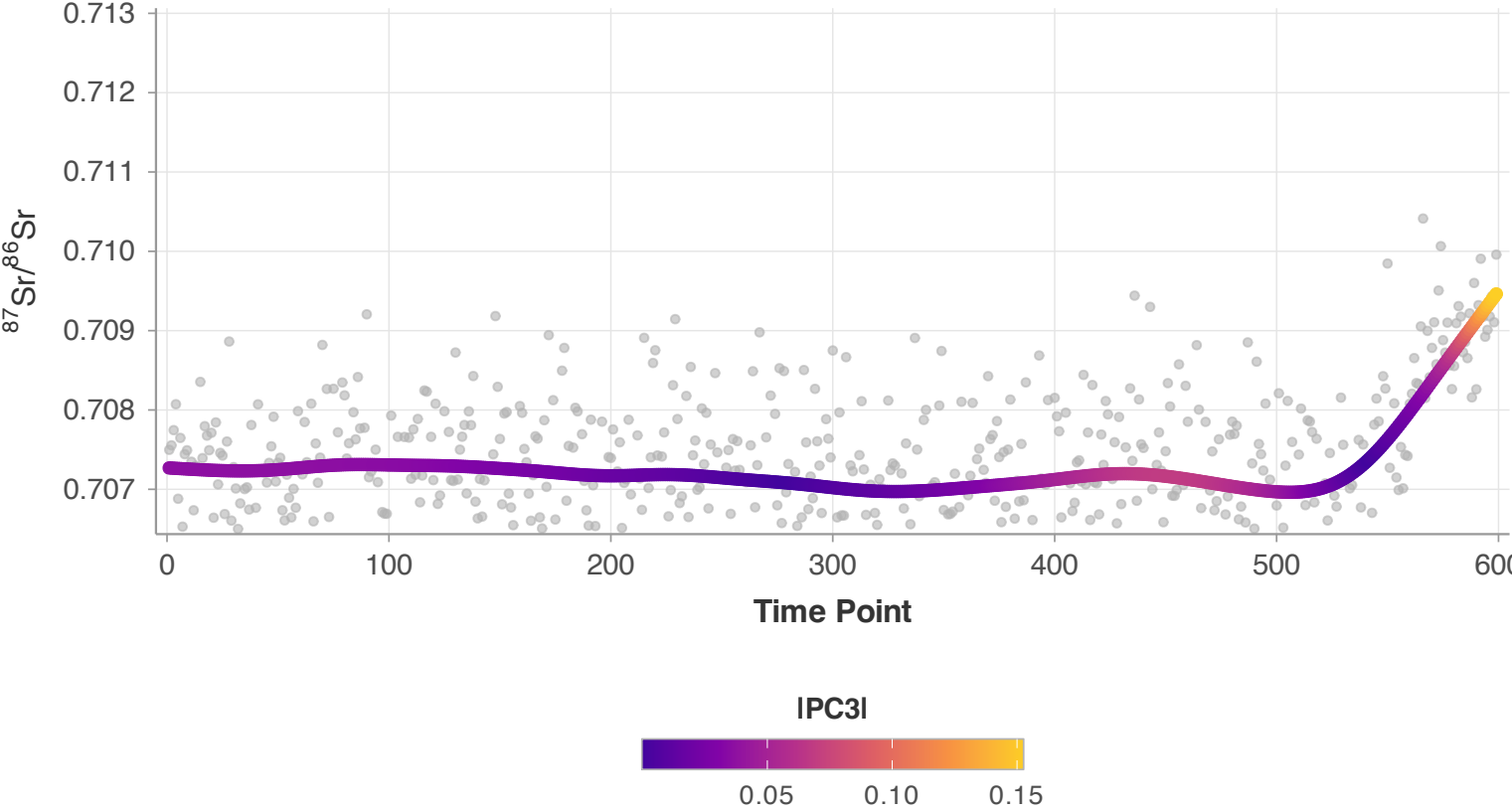
PC3 (1.7%)
