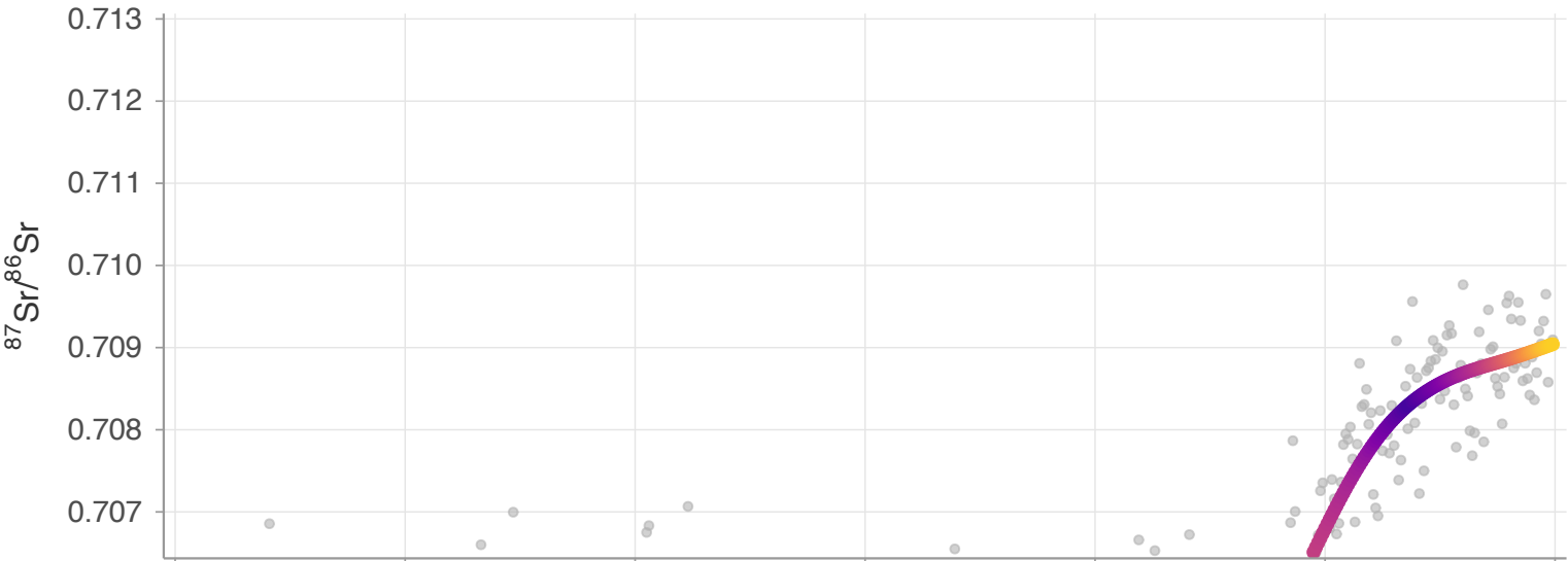
PC3 (1.1%)
