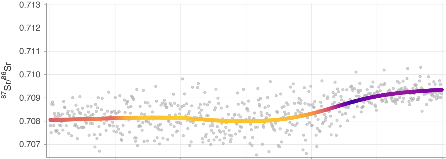
PC1 (47.5%)
