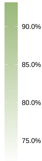
F1-Score
