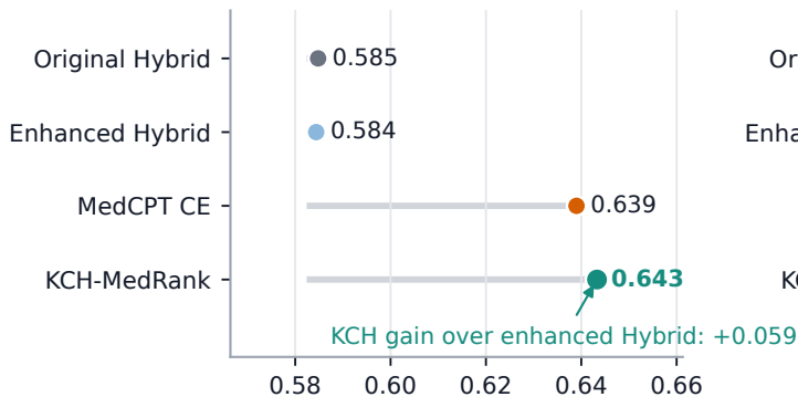
nDCG@10
