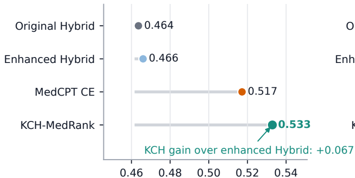
nDCG@10
