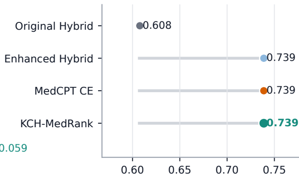
Recall@100
