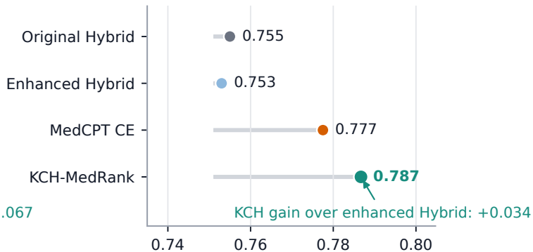
Recall@100
