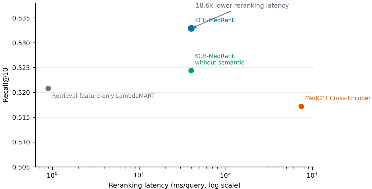
Efficiency-performance tradeoff on BioASQ
