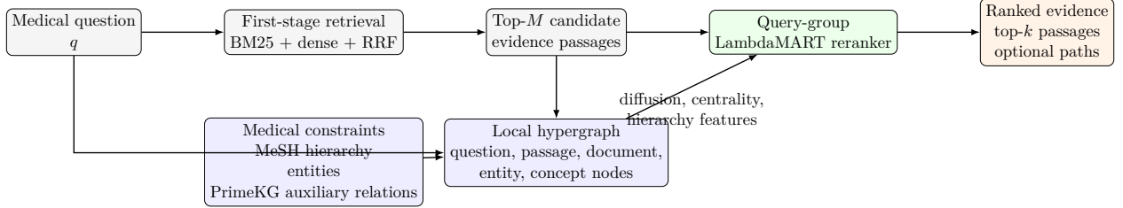
Figure 1: Overview of KCH-MedRank. The method first builds a high-recall candidate pool, constructs a local knowledge-constrained hypergraph around each question and candidate set, and uses hypergraph and biomedical semantic features in query-group learning-to-rank.
