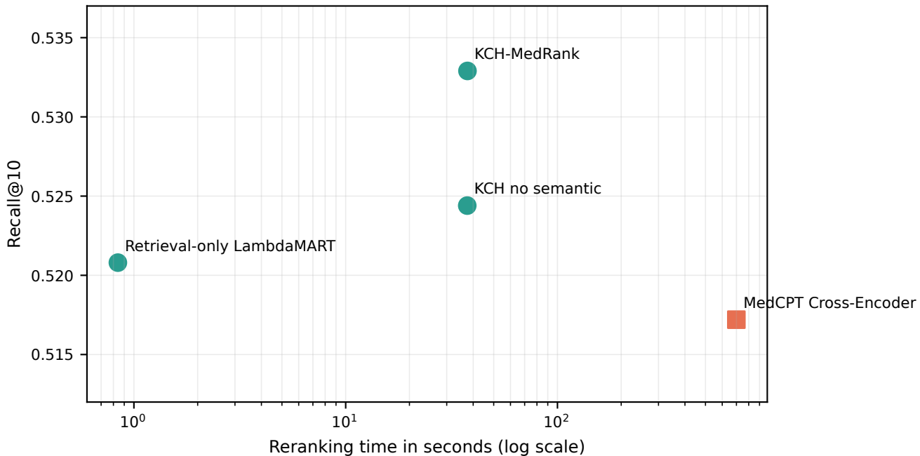
Reranking-stage efficiency versus evidence coverage
