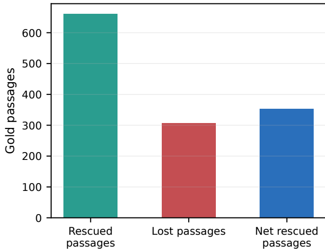
Passage-level rescue balance
