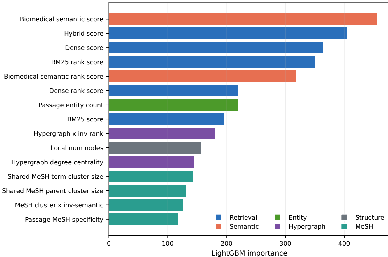
Top KCH-MedRank feature importances
