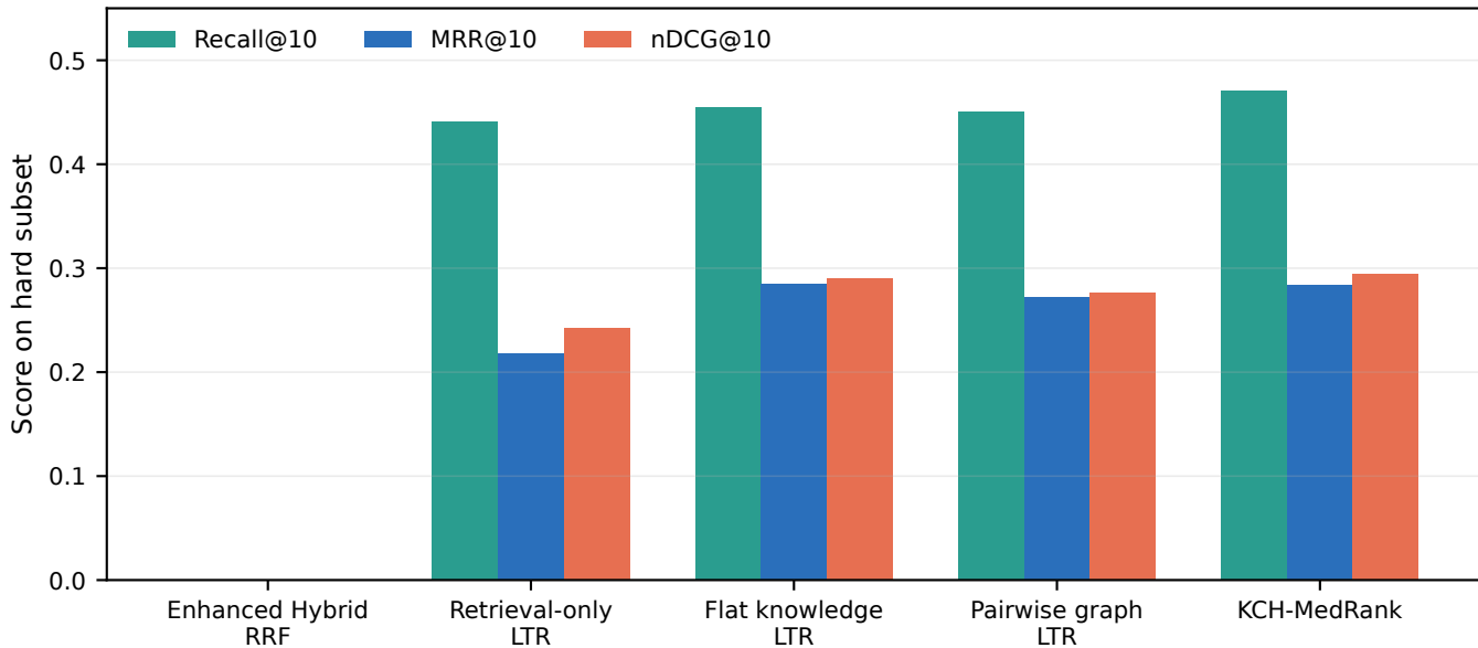
Recovering missed top-10 evidence when gold is in top-100
