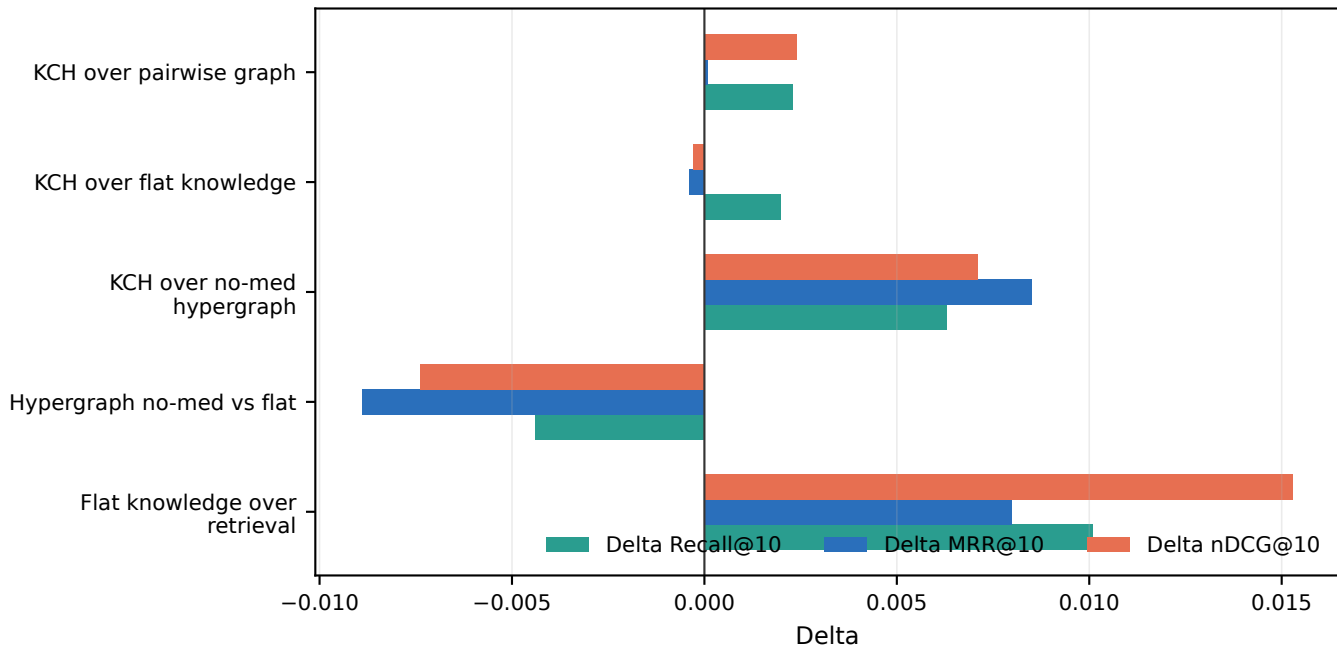
Structural ablation deltas on BioASQ
