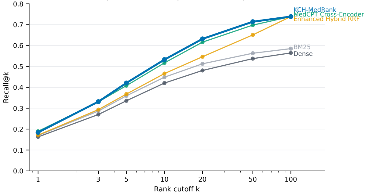
Recall improves across early and candidate-pool ranks
