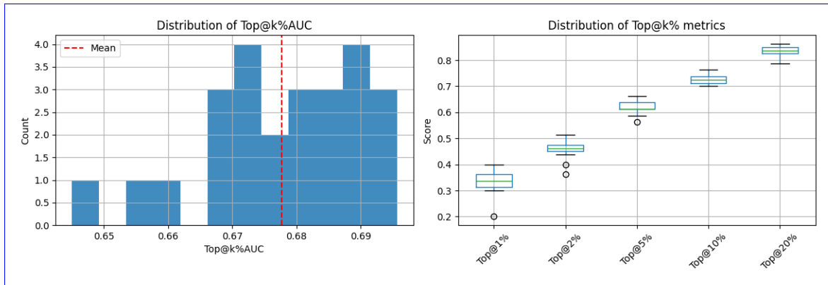
FIGURE 12. Distribution of test-set metrics of CatBoost + ES across 25 independent retraining runs. Each run uses a different random 70% subset of the training cross-sections; the validation and test sets are held fixed. Left: histogram of Top@ k\% AUC (integrated and normalized over k\% \in (0, 20\%] ) across the 25 runs; the vertical dashed line is the across-run mean. Right: box plots of Top@ k\% at k\% \in \{1, 2, 5, 10, 20\} . Takeaway: \sigma_{\text{Top@}k\%\text{AUC}} = 0.013 and the central 80% of runs fall in [0.662, 0.693] .
