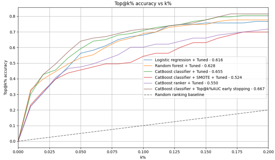
FIGURE 5. Top@k% accuracy and Top@k%AUC on the validation sample. CatBoost + ES has the largest validation Top@k%AUC (0.667) and is selected for the final test portfolio.
