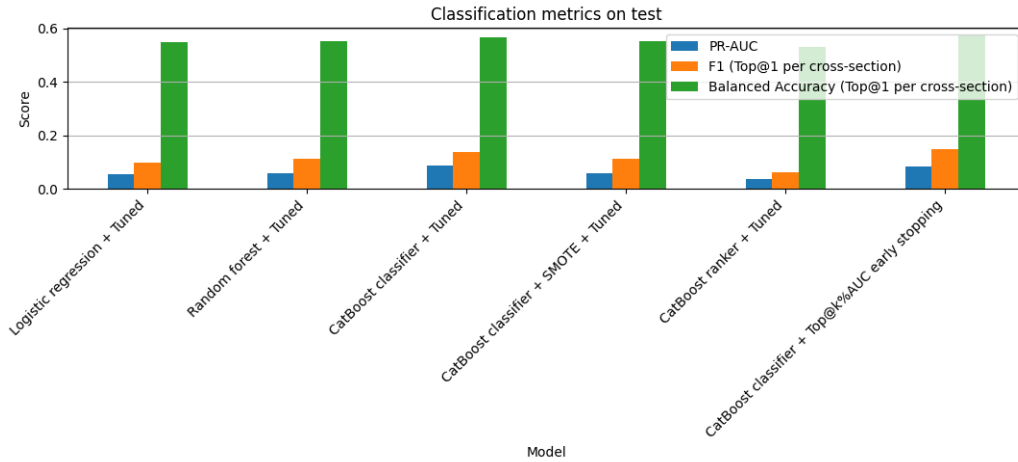
FIGURE 9. Standard classification metrics on the test set for all tuned models and CatBoost + ES. Each grouped bar reports Precision-Recall AUC (left), F1-score under a Top@1-per-cross-section decision rule (middle), and balanced accuracy, the average of sensitivity and specificity (right). PR-AUC is preferred over ROC-AUC under the \sim 1:287 class imbalance.
