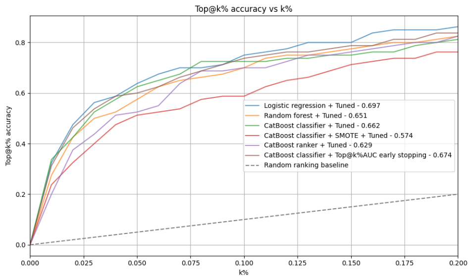
FIGURE 8. Top@ k\% accuracy on the test sample, normalizing the portfolio size by the cross-section size to control for its growth over time. The horizontal axis is the fraction k\% of the cross-section retained; the vertical axis is the probability that the target is covered.
