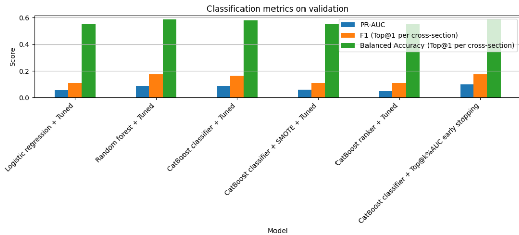
FIGURE 6. PR-AUC, F1, and balanced accuracy on the validation sample. F1 and balanced accuracy use the Top@1-per-cross-section decision rule.
