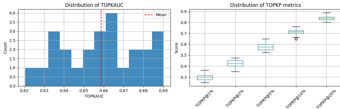
FIGURE 9. Distribution of test-set metrics of CatBoost + ES across 25 independent retraining runs. Each run uses a different random 70% subset of the training cross-sections; the validation and test sets are held fixed. Left: histogram of TOPKAUC (integrated and normalized over K\% \in \{0, 20\%\} ) across the 25 runs; the vertical dashed line is the across-run mean. Right: box plots of TOPKP at K\% \in \{1, 2, 5, 10, 20\} . Takeaway: \sigma_{\text{TOPKAUC}} = 0.020 and 80% of runs fall in [0.635, 0.685] , so the headline performance is not driven by a fortunate training-set composition.
