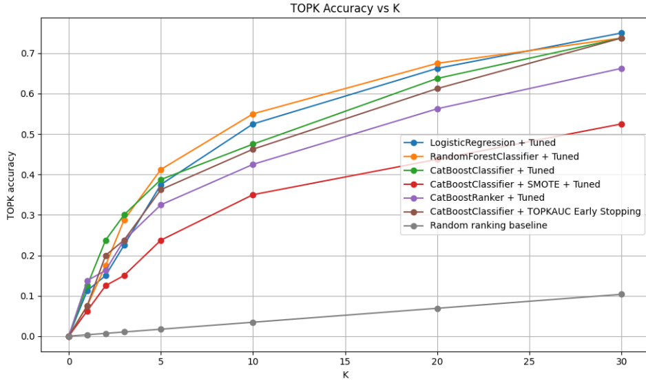
FIGURE 4. TOPK accuracy on the test sample for all models and the random-ranking baseline. The horizontal axis is the portfolio size K ; the vertical axis is the empirical probability that the manipulation target appears among the K highest-scored assets.
