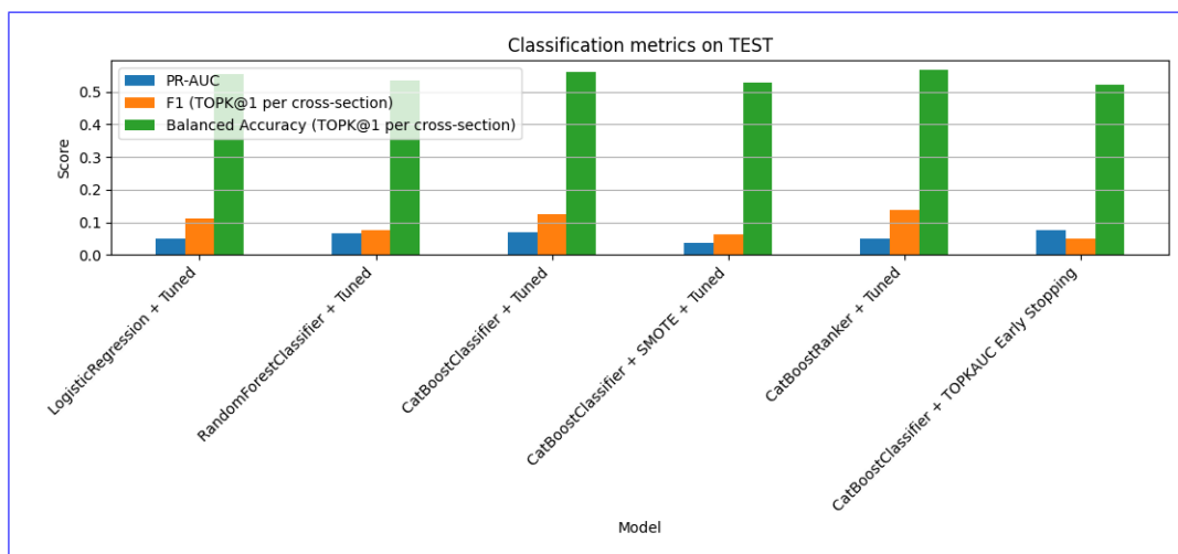
FIGURE 6. Standard classification metrics on the test set for all tuned models and CatBoost + ES. Each grouped bar reports Precision-Recall AUC (left), F1-score under a TOPK@1-per-cross-section decision rule (middle), and balanced accuracy, the average of sensitivity and specificity (right). PR-AUC is preferred over ROC-AUC under the \sim 1:290 class imbalance. Takeaway: the two imbalance-aware CatBoost variants dominate the standard classification measures as well as the ranking metrics, ruling out a calibration artefact.
