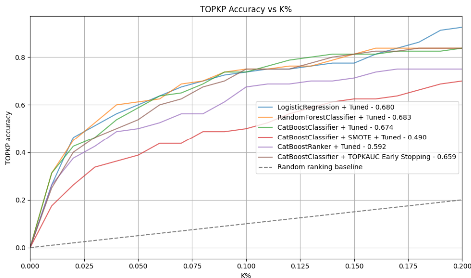
FIGURE 5. Top@K% of models TOPKP accuracy on the test sample, normalizing the portfolio size by the cross-section size to control for its growth over time. The horizontal axis is the fraction K% of the cross-section retained; the vertical axis is the probability that the target is covered.
