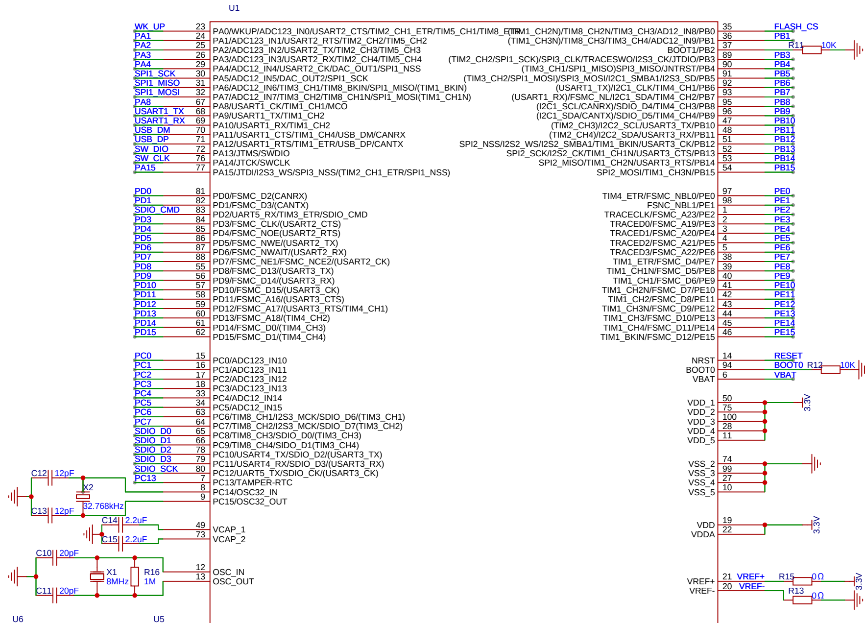
STM32F407VGT6
