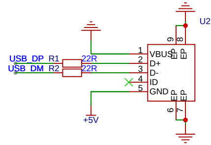
microUSB
