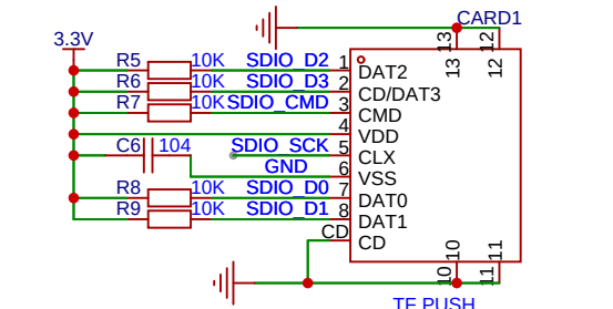
microSD
