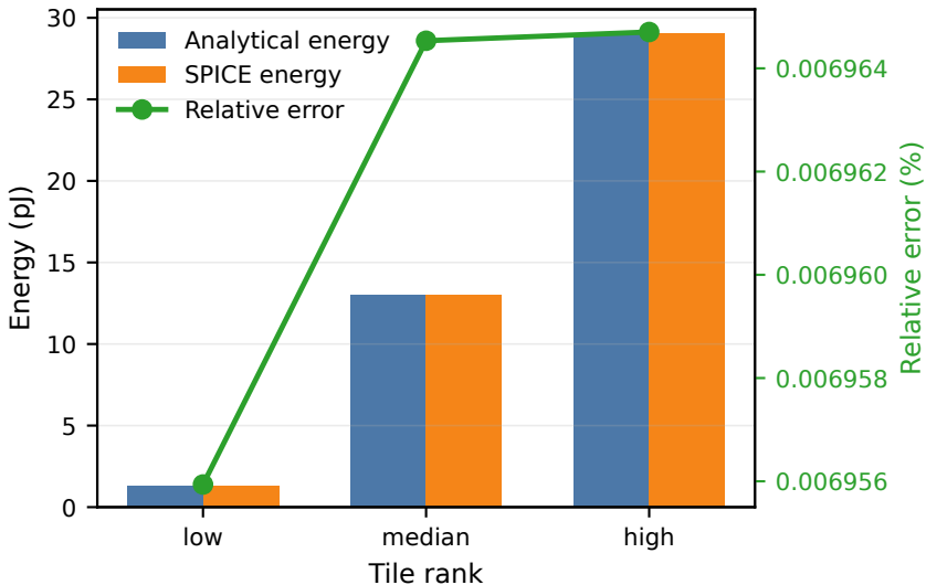
Analytical vs ngspice tile energy
