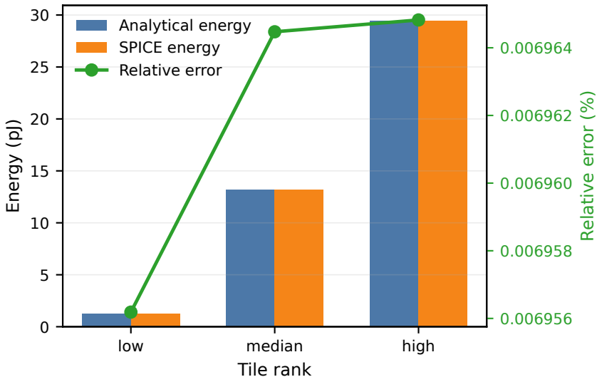
Analytical vs ngspice tile energy
