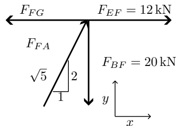
Figure 0.7: Free-body diagram of joint F .
