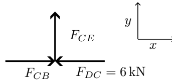
Figure 4: Free-body diagram of joint C .
