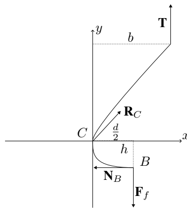
Figure 1: Free-body diagram of the right tong half
