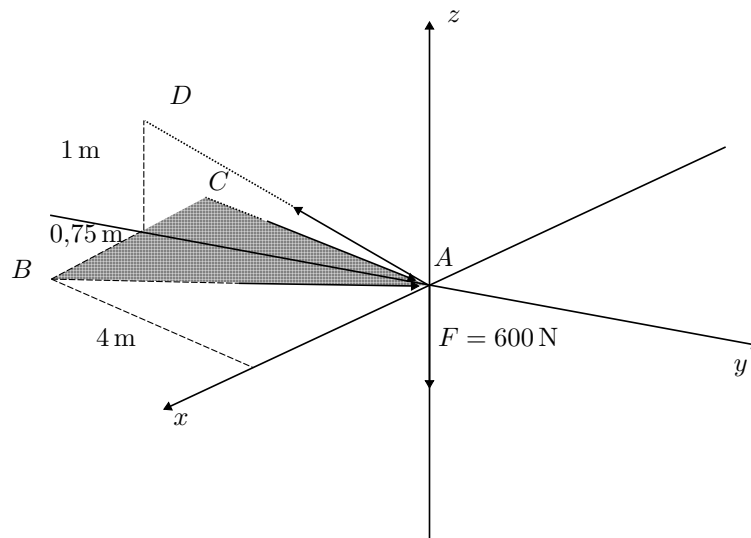
Figure 10: Free-body diagram of the space truss
