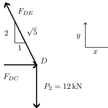
Figure 3: Free-body diagram of joint D .
