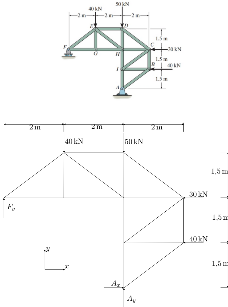
Figure 8: Free-body diagram for the entire truss.
