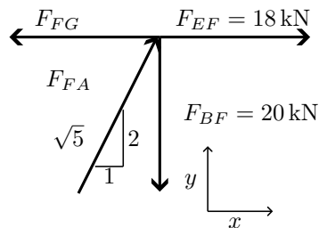
Figure 7: Free-body diagram of joint F .
