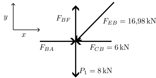
Figure 6: Free-body diagram of joint B .
