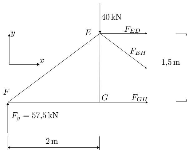
Figure 9: Free-body diagram of a section of the truss.
