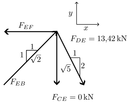
Figure 5: Free-body diagram of joint E .
