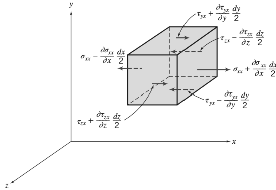
Figure 4.7: Stresses in the x direction on a fluid element.
