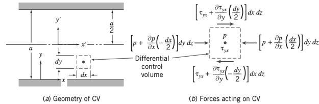
Figure 7.3: Control volume for analysis of laminar flow between stationary infinite parallel plates.
