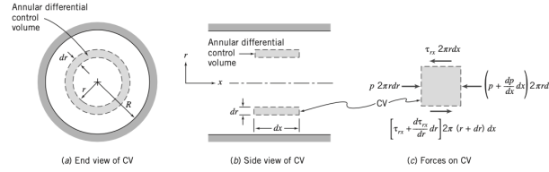
Figure 7.4: Differential control volume for analysis of fully developed laminar flow in a pipe.
