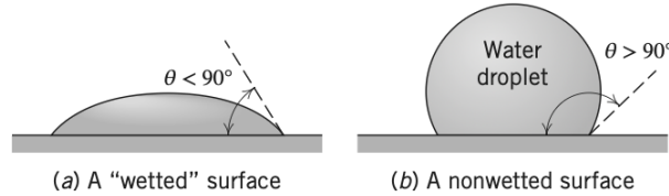
Figure 1.5: Surface tension effects on water droplets.
