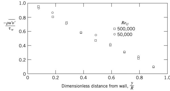
Figure 7.5: Turbulent shear stress (Reynold's stress) for fully developed turbulent flow in a pipe.
