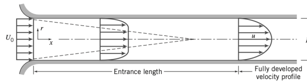
Figure 7.1: Flow in the entrance region of a pipe.
