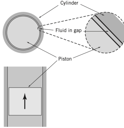
Figure 7.2: Piston-cylinder system approximated as infinite parallel plates.
