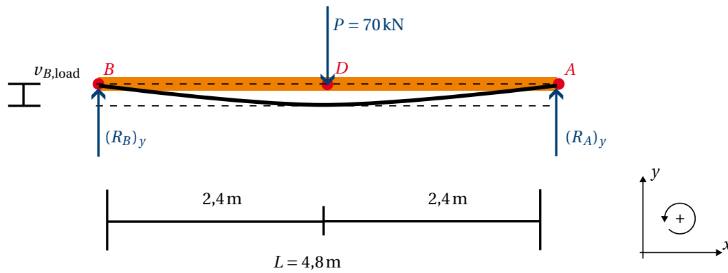
Figure 4.3: Free body diagram of the deflection of member AB .
