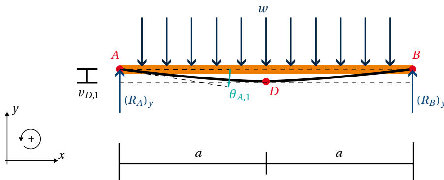
Figure 3.1: Free Body diagram of the simply supported beam AB .
