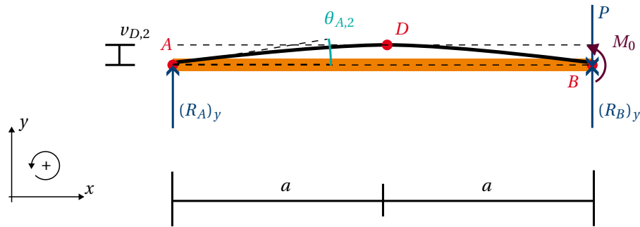
Figure 3.2: Free Body diagram of the contribution from the overhang BC.
