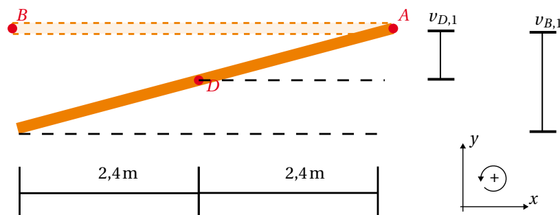
Figure 4.2: Free Body diagram of the rigid rotation of member AB .
