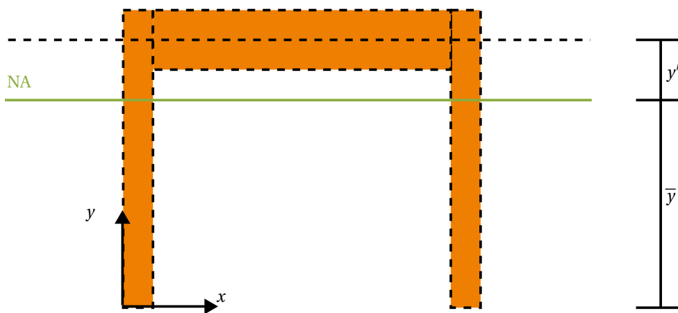
Figure 6.2: Cross section of the composite beam showing the position of the neutral axis, NA.
