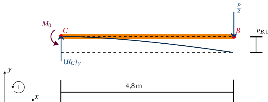
Figure 4.1: Free Body diagram of the cantilevered beam BC .
