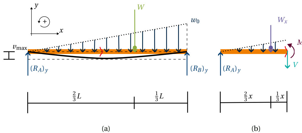
Figure 1.1: (a) Free body diagram of the beam and (b) a cut of said beam taken at a distance x .
