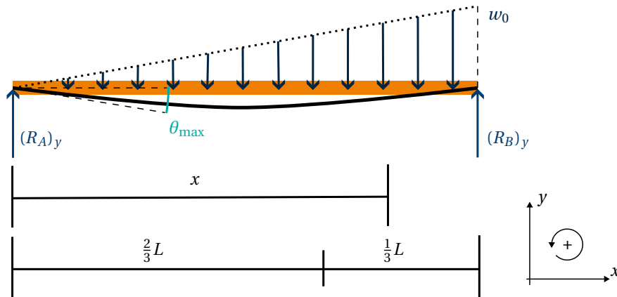
Figure 2.1: Free body diagram of the beam.
