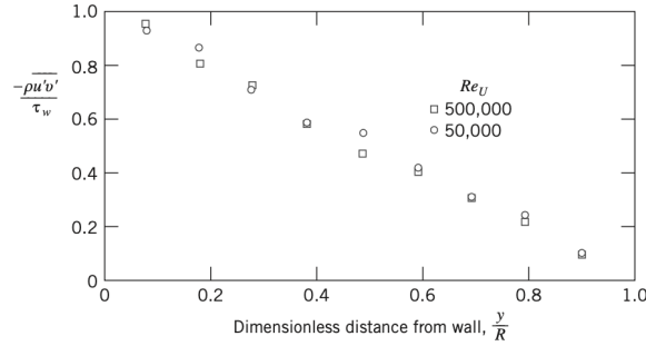
Figure 18.1: Turbulent shear stress (Reynold's stress) for fully developed turbulent flow in a pipe.
