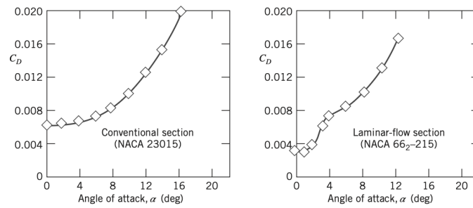
Figure 21.10: Drag Coefficient versus angle of attack for two airfoil sections of 15% thickness ratio at Re_c = 9 \cdot 10^6 .
