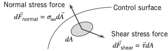
Figure 7.2: Normal and shear stress forces.
