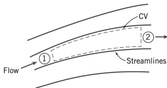
Figure 13.1: Flow through a stream tube.
