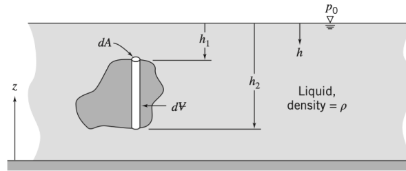
Figure 4.2: Immersed body in a static liquid.
