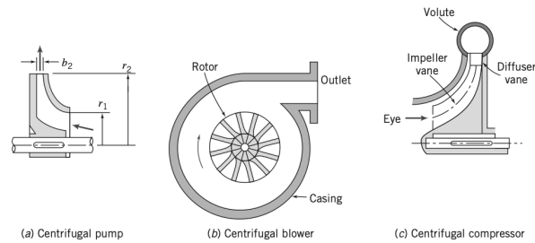
Figure 23.1: Schematic of typical centrifugal-flow turbomachines.
