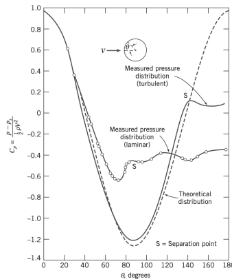
Figure 21.6: Pressure distribution around a smooth sphere for laminar and turbulent boundary-layer flow, compared with inviscid flow.
