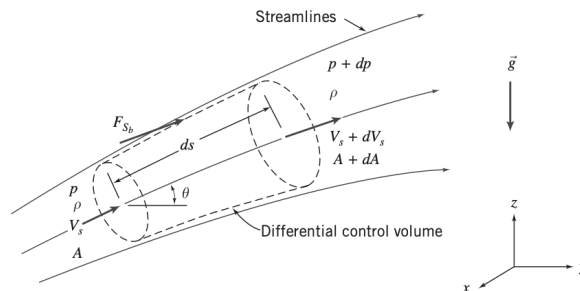
Figure 7.1: Differential control volume through a stream tube.
