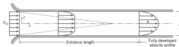
Figure 17.1: Flow in the entrance region of a pipe.
