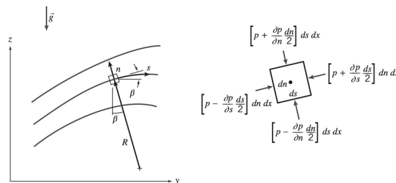
Figure 12.1: Fluid particle moving along a streamline.
