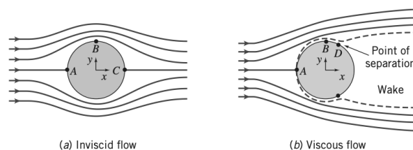
Figure 2.6: Incompressible flow over a sphere
