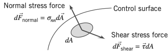
Figure 7.2: Normal and shear stress forces.
