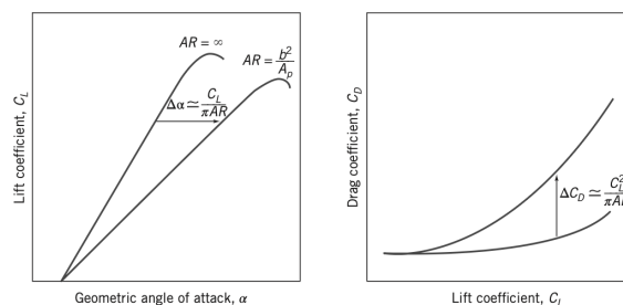
Figure 21.12: Effect of finite aspect ratio on lift and drag coefficients for a wing.
