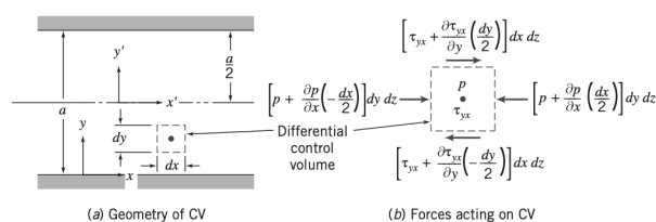
Figure 17.3: Control volume for analysis of laminar flow between stationary infinite parallel plates.
