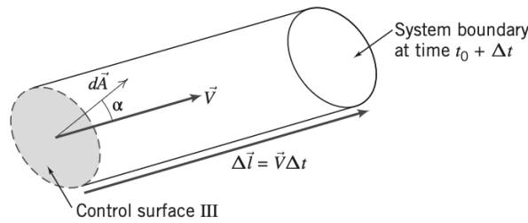
Figure 6.2: Enlarged view of subregion 3 from Figure 6.1
