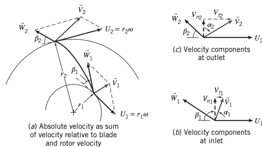
Figure 23.4: Geometry and notation used to develop velocity diagrams for radial-flow machines.
