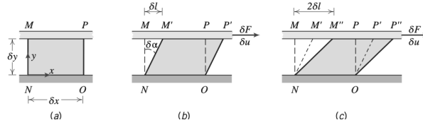
Figure 2.4: (a) Fluid element at time t , (b) deformation of fluid element at time t + \delta t , (c) deformation of fluid element at time t + 2\delta t
