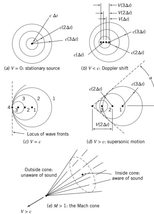
Figure 25.2: Propagation of sound waves from a moving source: The Mach cone.
