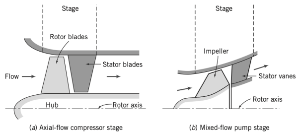
Figure 23.2: Schematic of typical axial- and mixed-flow turbomachines
