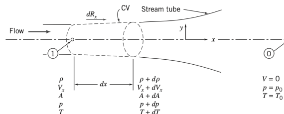
Figure 25.4: Compressible flow in an infinitesimal stream tube.
