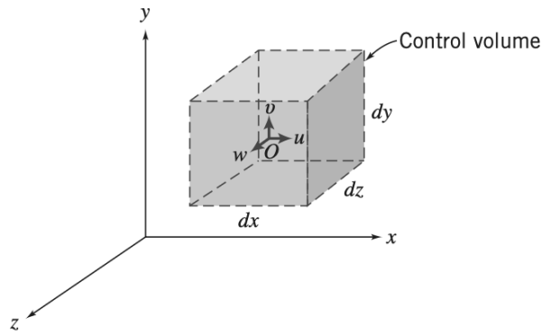
Figure 9.1: Differential control volume in rectangular coordinates.
