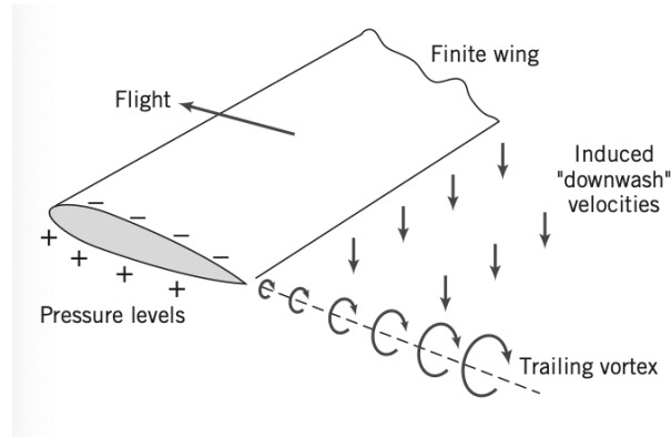
Figure 21.11: Schematic representation of the trailing vortex system of a finite wing.
