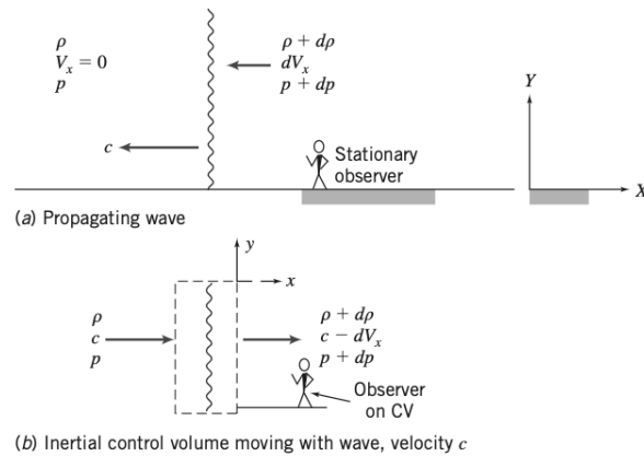
Figure 25.1: Propagating sound wave showing control volume chosen for analysis.
