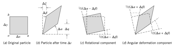
Figure 10.3: Rotation and angular deformation of perpendicular line segments in a two-dimensional flow.
