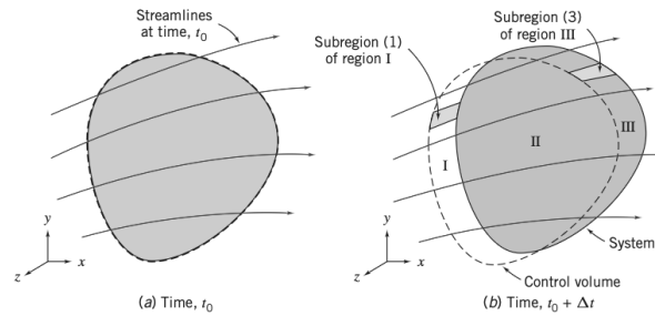
Figure 6.1: Configuration of the system and control volume.
