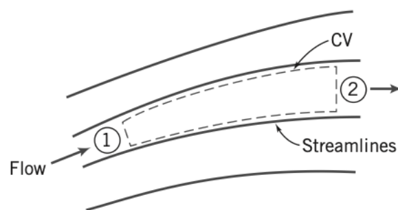
Figure 13.1: Flow through a stream tube.
