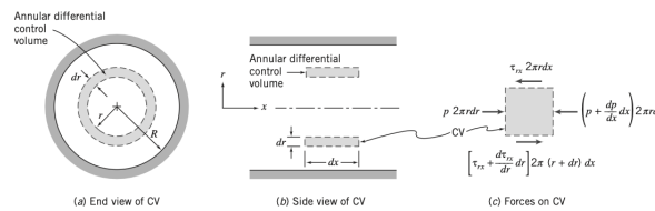
Figure 17.4: Differential control volume for analysis of fully developed laminar flow in a pipe.
