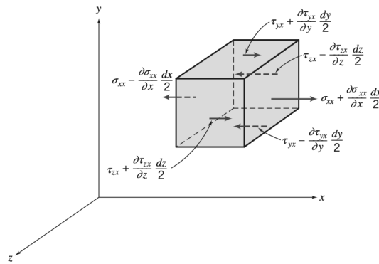
Figure 10.5: Stresses in the x direction on a fluid element.
