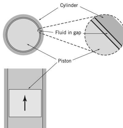
Figure 17.2: Piston-cylinder system approximated as infinite parallel plates.
