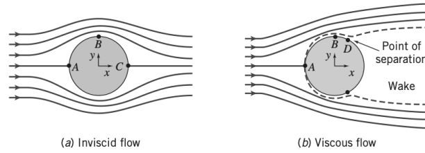
Figure 1.6: Incompressible flow over a sphere
