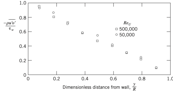
Figure 7.5: Turbulent shear stress (Reynold's stress) for fully developed turbulent flow in a pipe.
