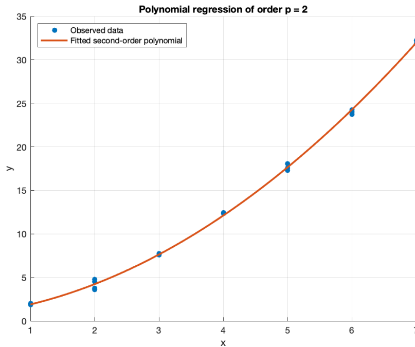
Figure 2: Fitted second-order polynomial for problem 2.
