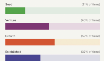
Fig. 7 Proportion of London companies that are actively hiring, by stage of evolution
