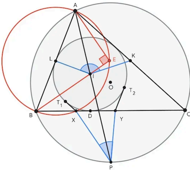
A TYPICAL GEOMETRY PROBLEM DIAGRAM IN AN IMO EXAM.
