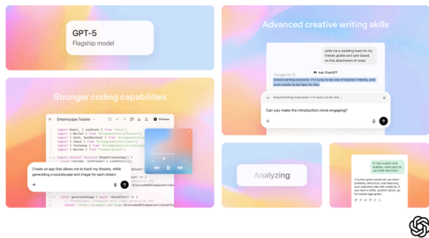
IMAGE CREDITS:OPENAI
