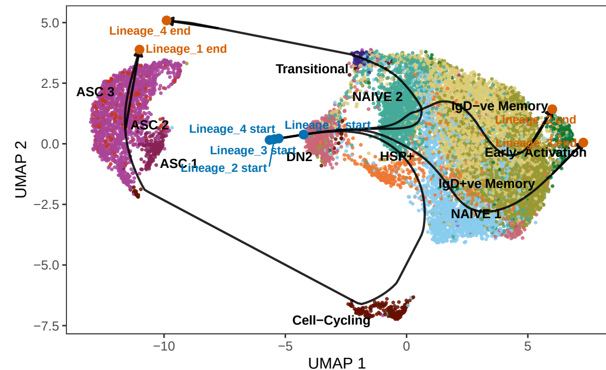
Slingshot trajectory coloured by annotated B-cell states
