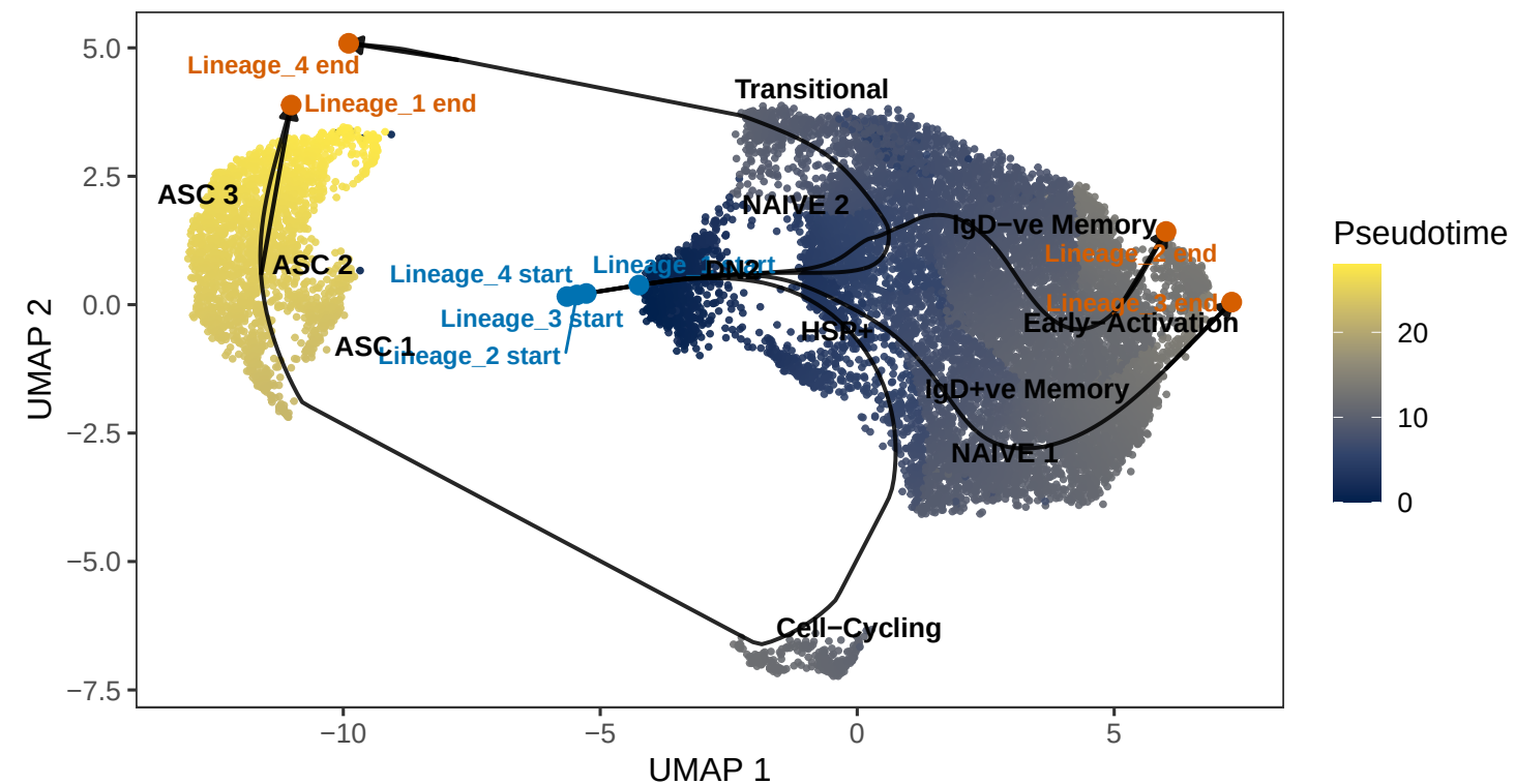
Slingshot trajectory coloured by pseudotime with cell type labels
