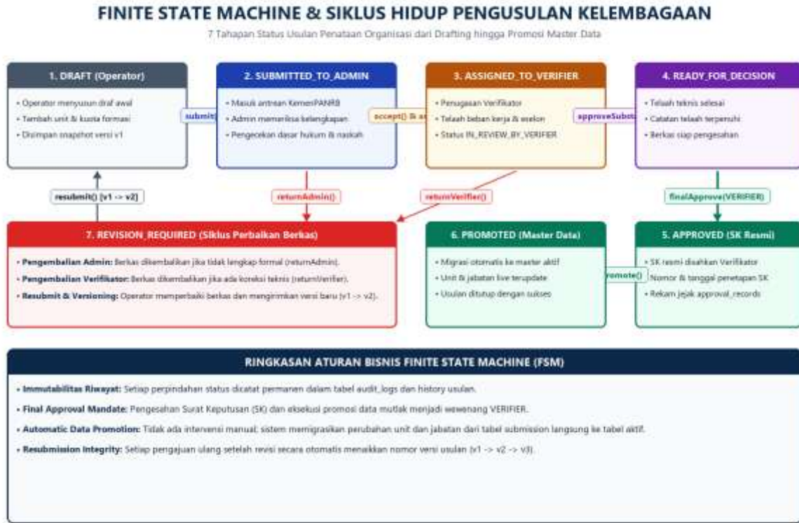
Gambar 7: Diagram Finite State Machine Siklus Hidup Pengusulan Kelembagaan
