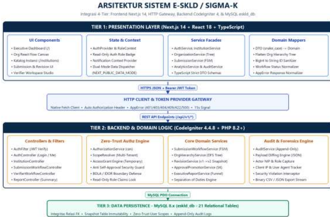
Gambar 1: Arsitektur Sistem Terintegrasi E-SKLD / SIGMA-K (4-Tier Architecture)
