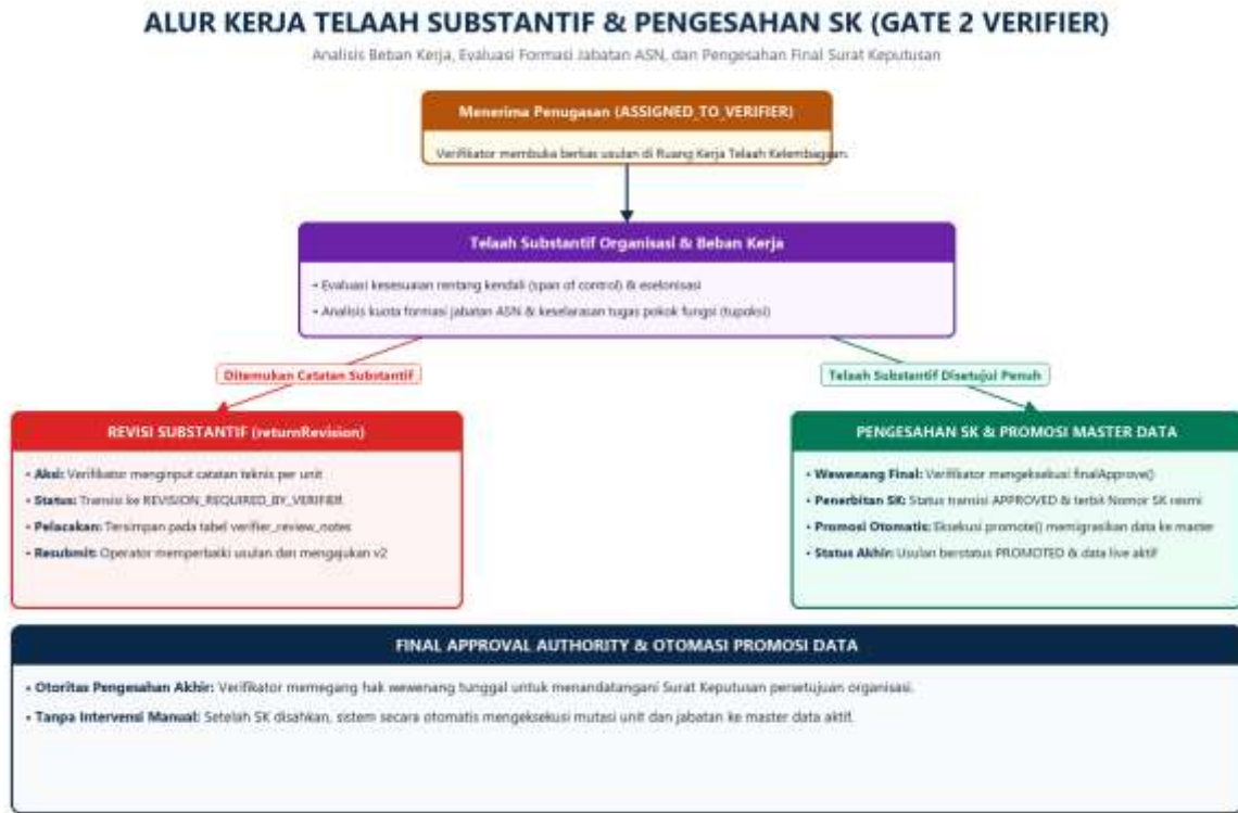
Gambar 10: Diagram Alir Kerja Telaah Substantif & Pengesahan SK (Gate 2 Verifier Workspace)
