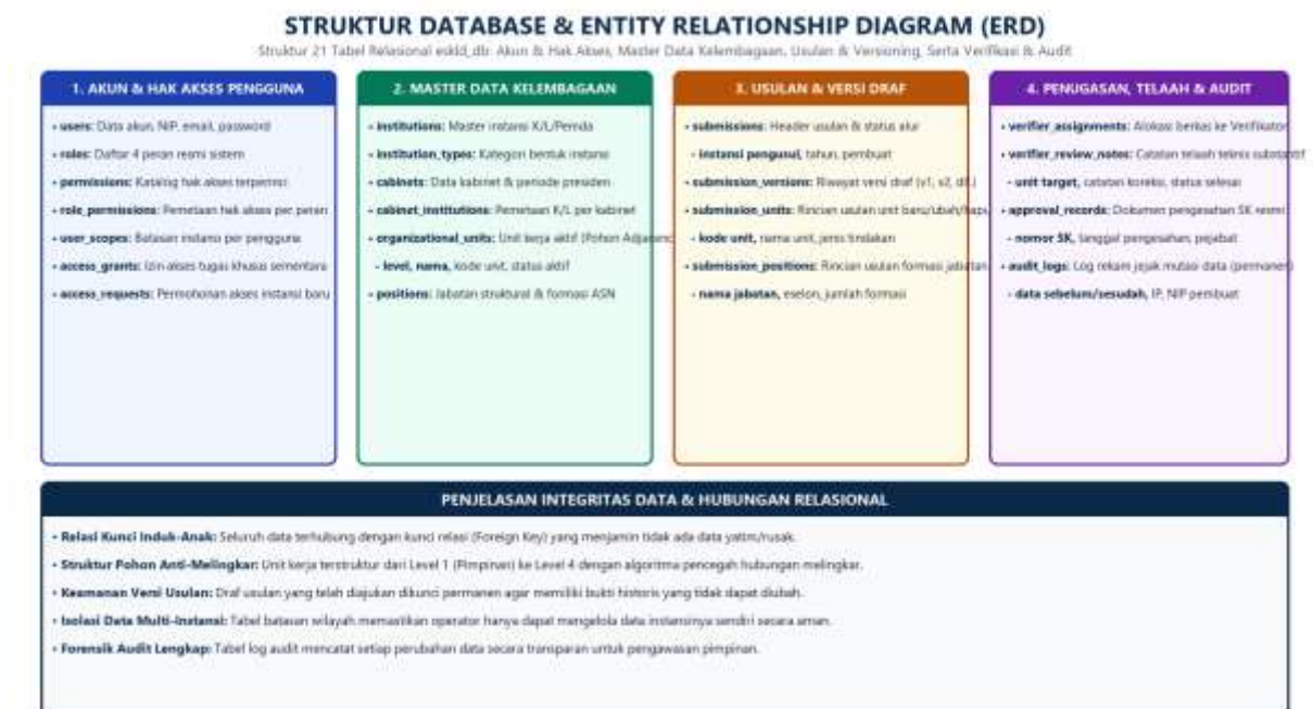
Gambar 6: Entity Relationship Diagram (ERD) Basis Data esklid_db (21 Tabel)
