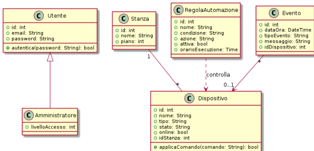
Figure 7: Classi dominio
