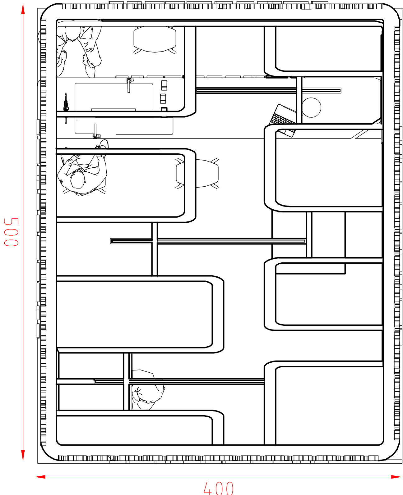
PLAN
