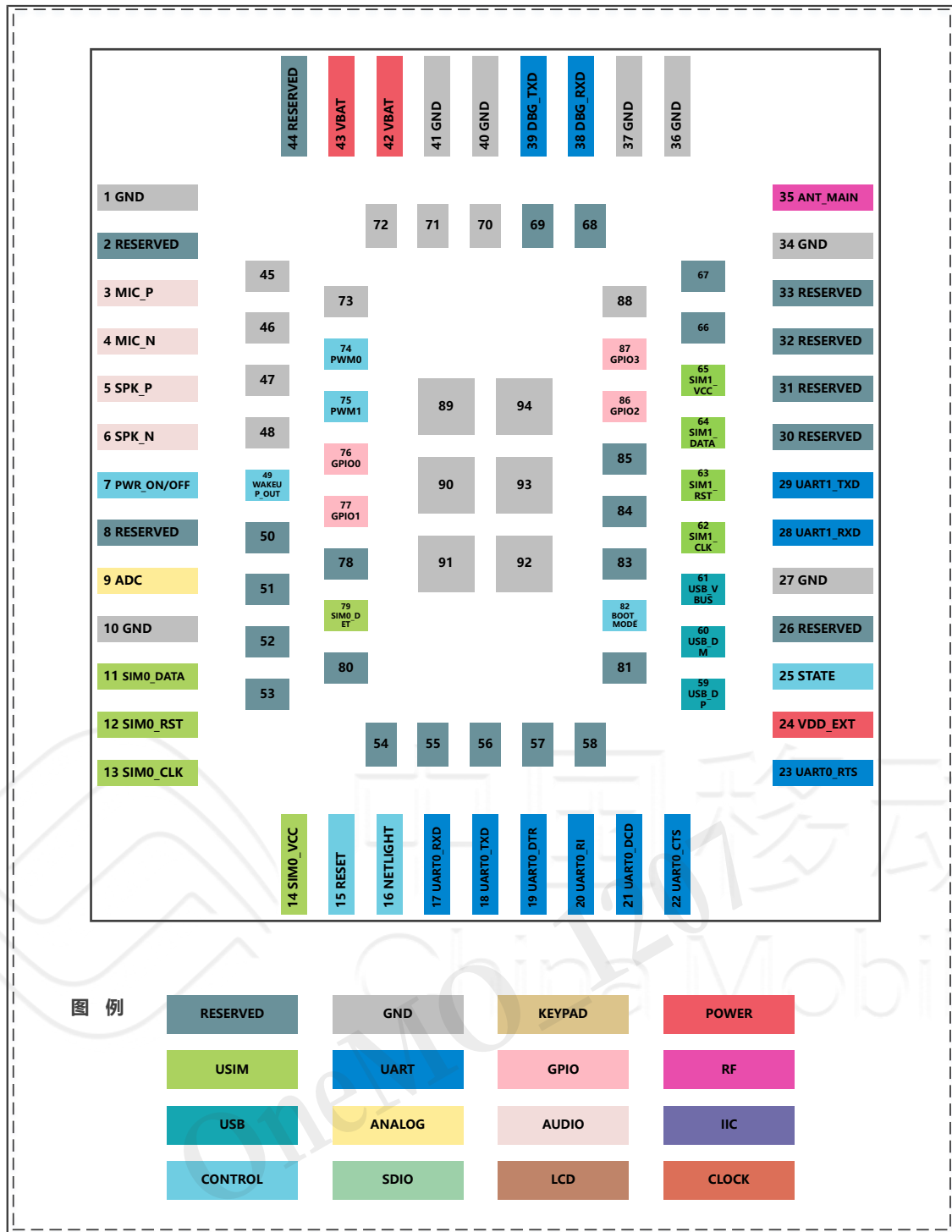
Figure 2. ML307A-D引脚分配图
