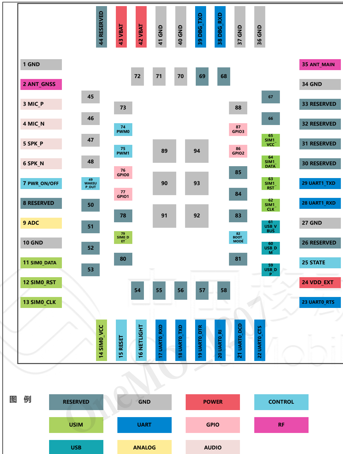
Figure 3. ML307A-G引脚分配图
