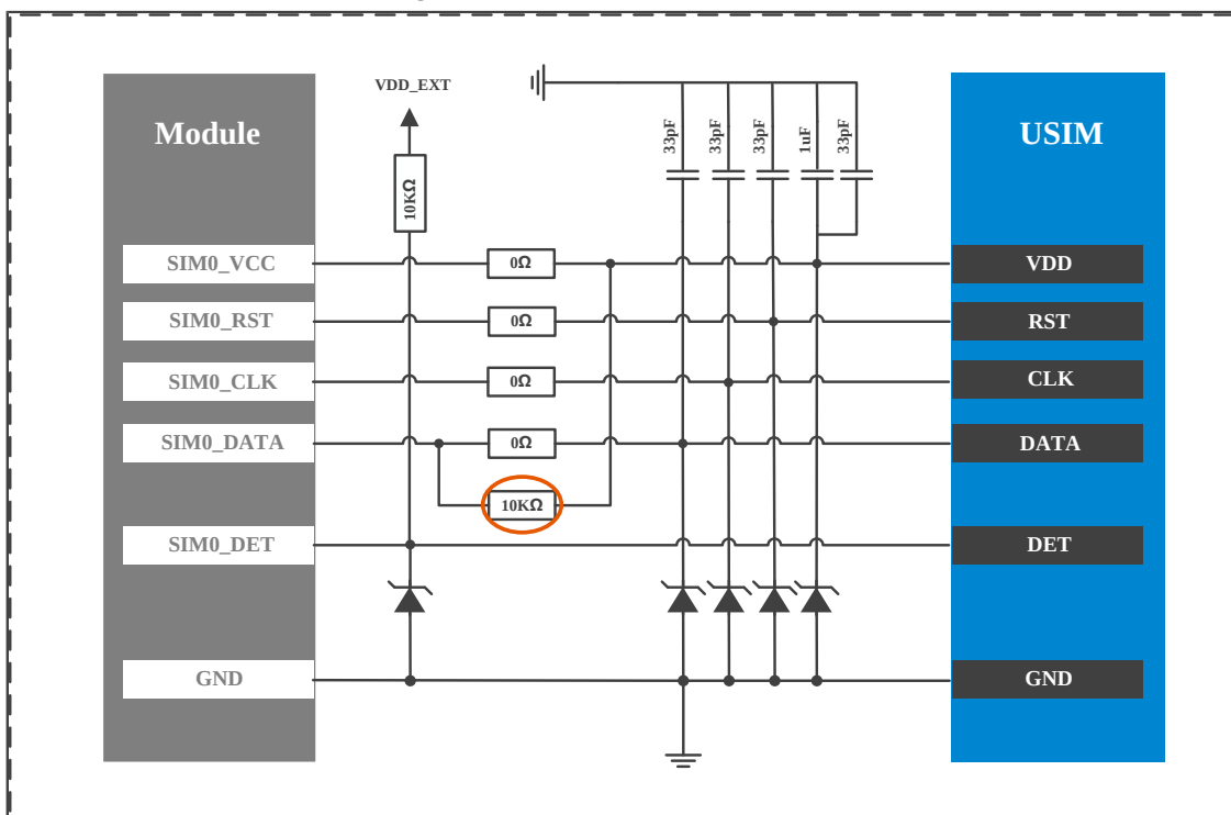
Figure 15. ML307A SIM0接口示意图
