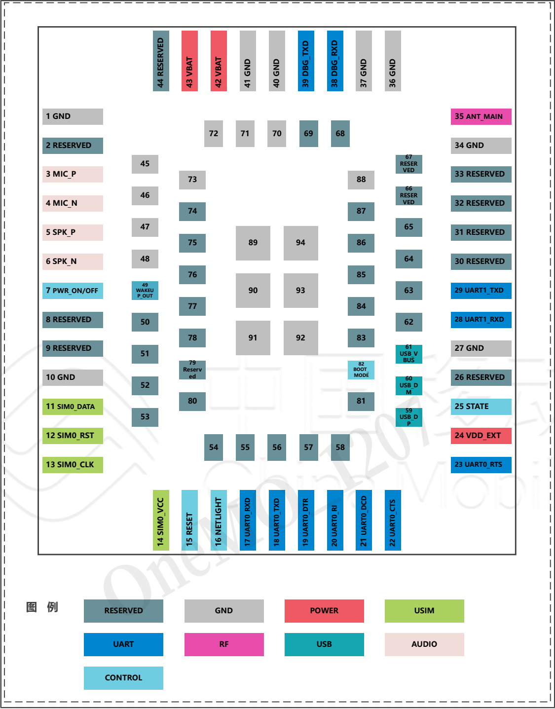
Figure 1. ML307S引脚分配图
