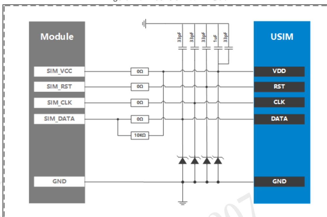
Figure 14. ML307S SIM接口示意图
