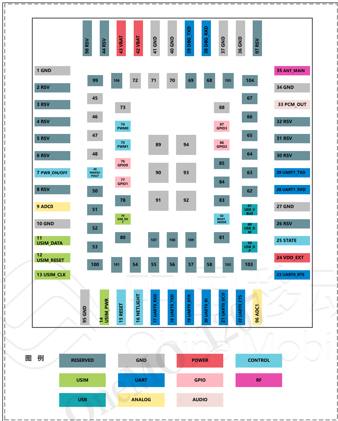
Figure 4. ML307R引脚分配图
