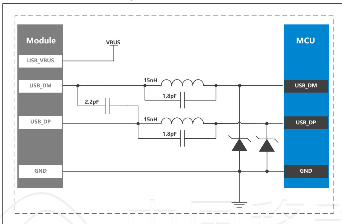
Figure 18. USB接口参考设计
