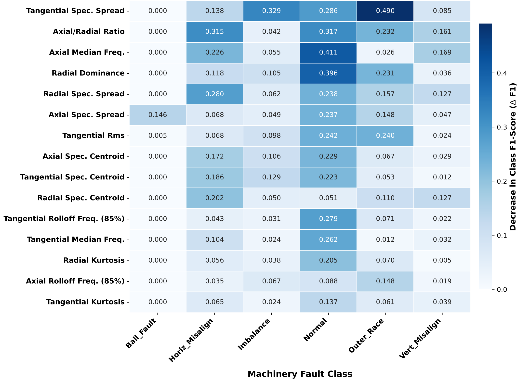
Directional Physics Alignment by Fault Type (Permutation Importance)
