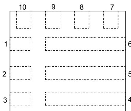
(QFN2.1X2.1-10)
